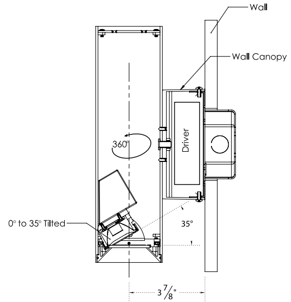
Wall Canopy
